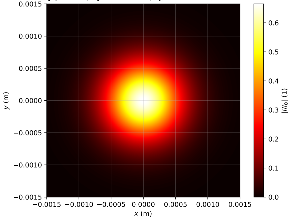
Intensity profile I(x, y, z = 2.229m)/I_0 , Pin=0.4Pcr, artificial time
